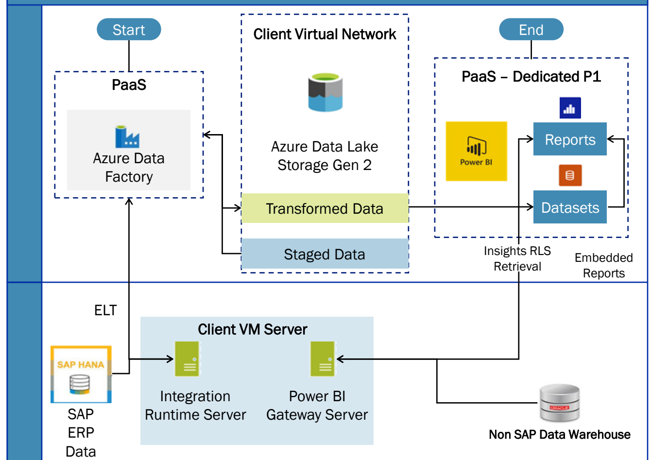
Typical SAP Landscape using Azure for example purposes
