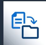
Document Classification
