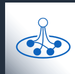
SAP Graph
