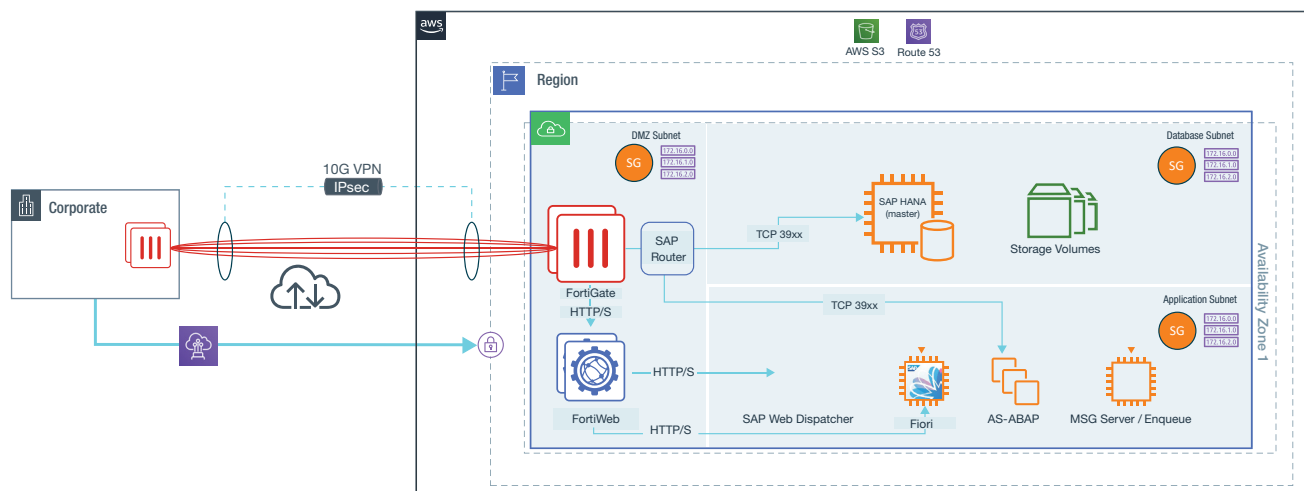
Figure 2: Fortinet Reference Architecture for SAP S/4HANA on AWS.
